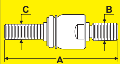
W-N14388 Ball Joint
